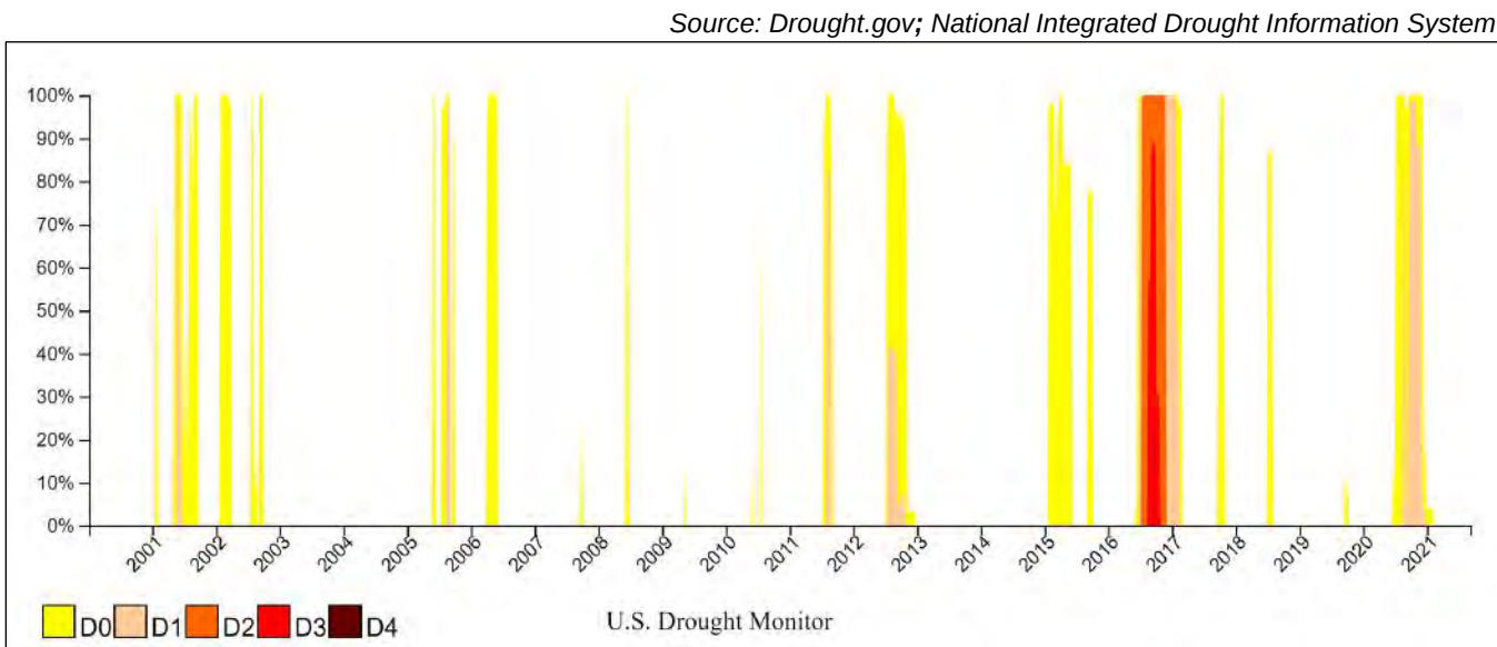
Figure 2. Historical Drought Severity—Percent of Tompkins County Experiencing Drought Level
